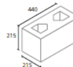
9" 2 Core Cavity Block
