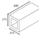
9" Cavity Block
