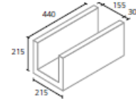
U-Block
